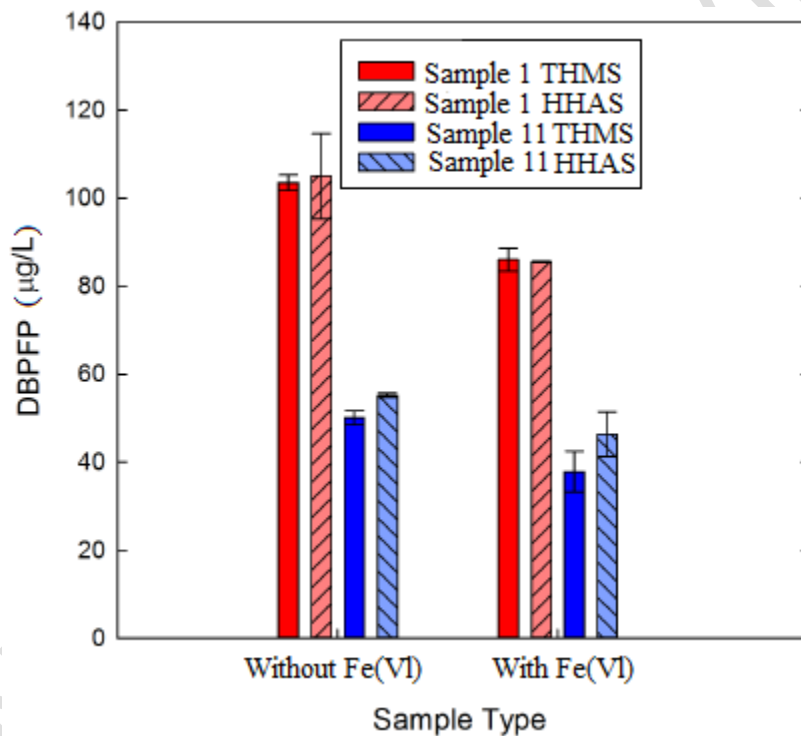
Fig. 3: Continuous flow DBPFP results for samples 1 and 11; for sample 1, \text{Fe(VI)} =25 \mu\text{M} and for sample 11, \text{Fe(VI)} =50 \mu\text{M}
