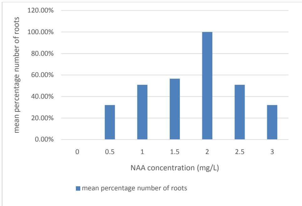
Figure 5: a graph showing NAA concentration against percentage number of roots
