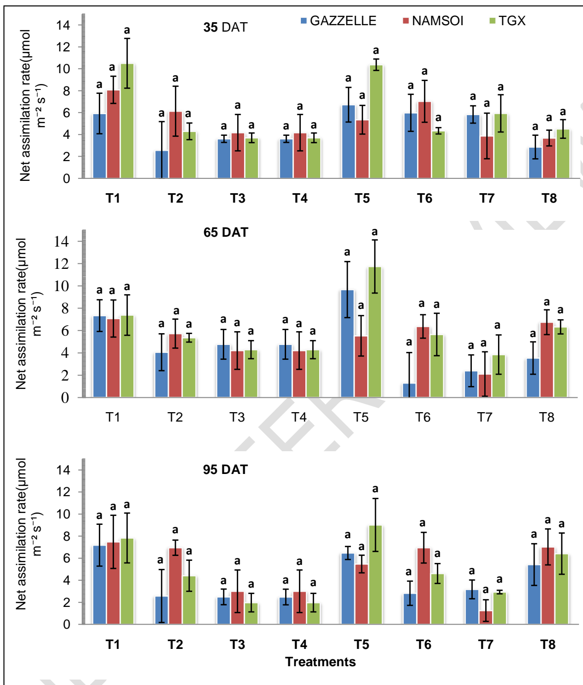
Fig. 2 Net photosynthetic CO 2 assimilation rate (A) in plants of the three soy bean genotypes on 35 DAT, 65 DAT and 95 DAT subjected to various treatments. Values are means of three replicates \pm SEs. Means with the same letter are not significantly different. Control (Water)*Inoculated (T1), 480 \mu\text{M} Al*Inoculated (T2), 750 \mu\text{M} Al*Inoculated (T3) and 960 \mu\text{M} Al*Inoculated (T4), Control (T5), 480 \mu\text{M} Al (T6), 750 \mu\text{M} Al (T7) and 960 \mu\text{M} Al (T8).
