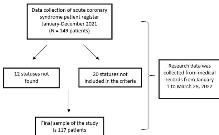
Fig. 1. Sampling process
