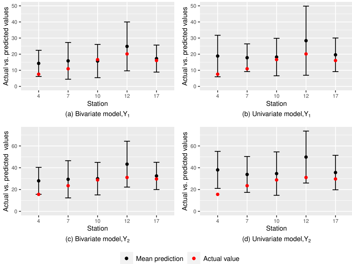
Figure 2: Predictions (mean \pm standard deviation) from the bivariate and univariate STAMs for the randomly selected five locations.
