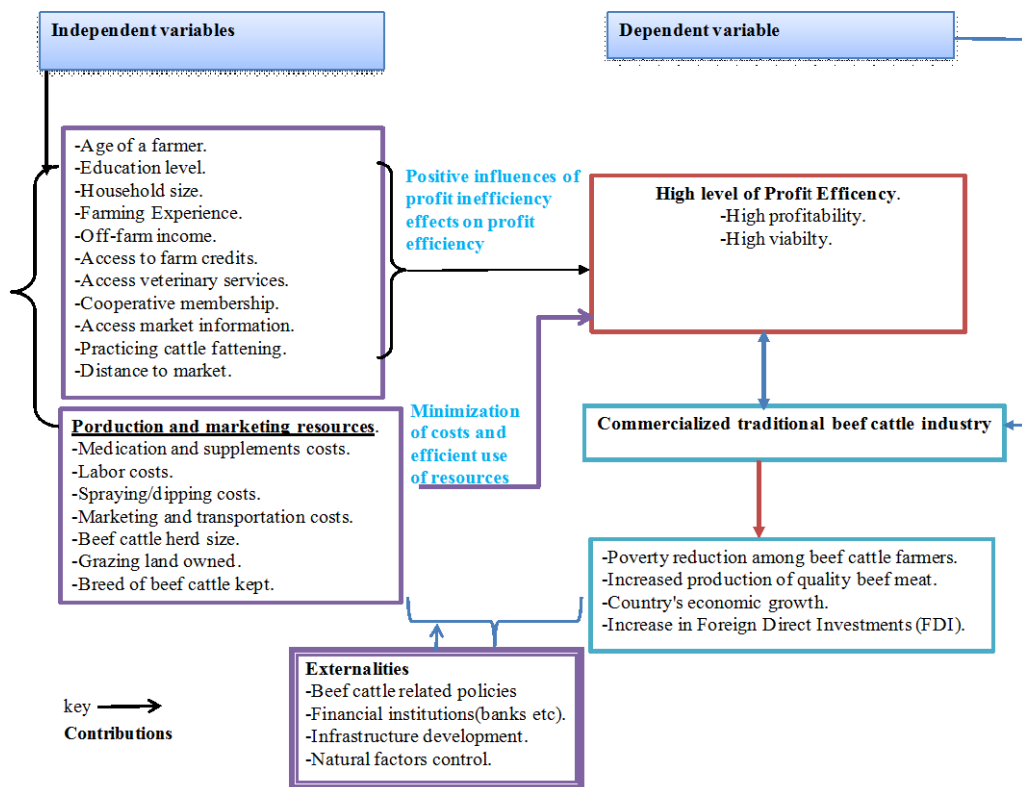
Fig 1. Conceptual framework.
