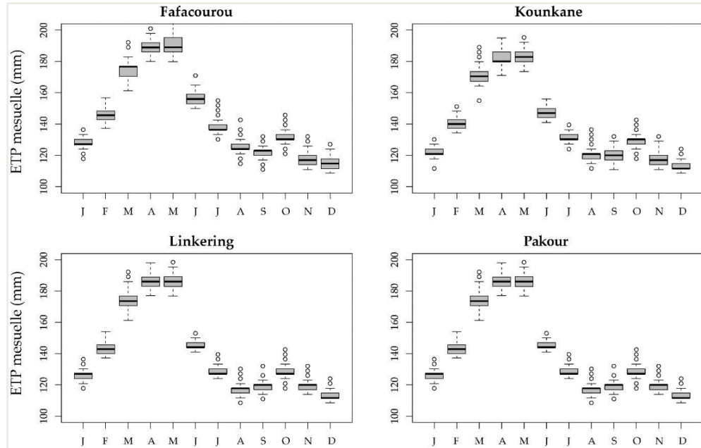
Figure 9. Seasonal cycle of the ETP of some stations of the Kayanga basin Improve the legibility of your Charts
