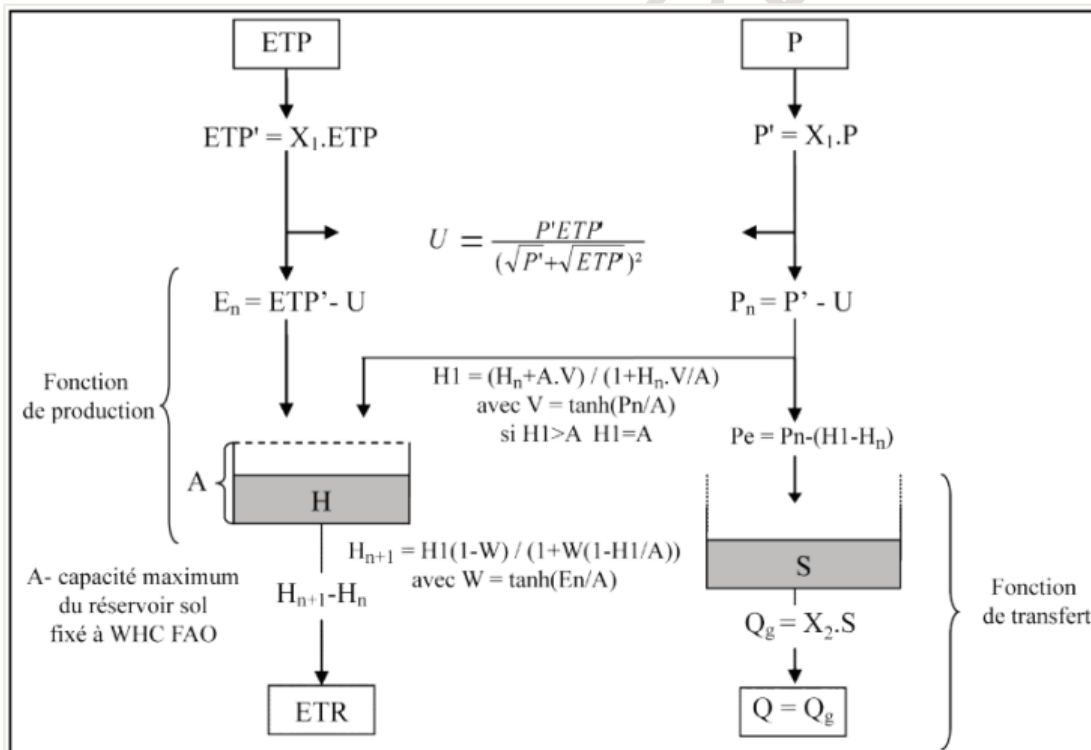
Figure 7: Conceptual diagram of the GR2M model (Bodian et al., 2012)
