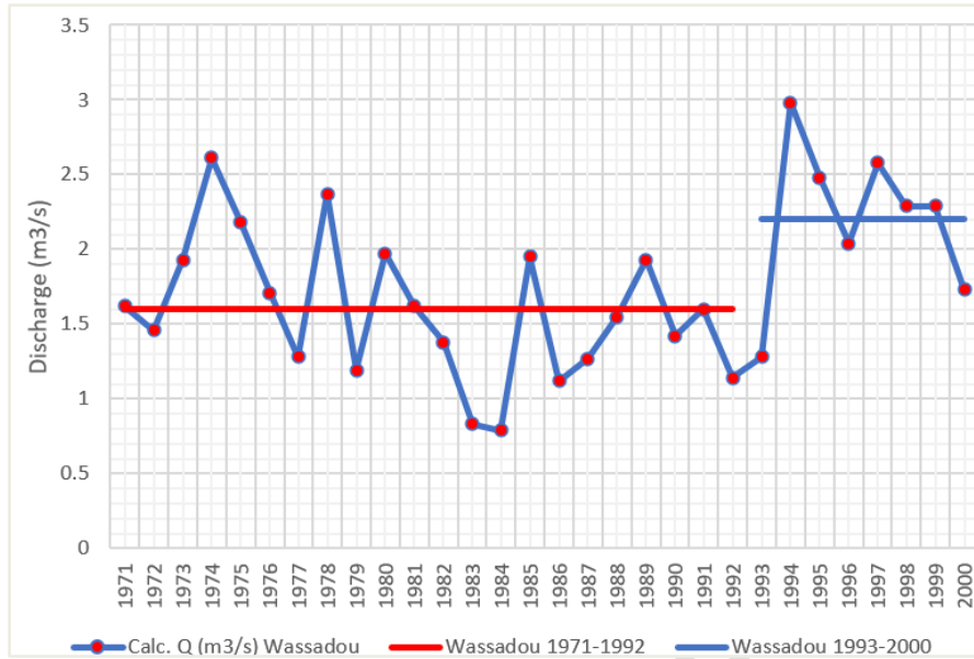
Figure 16. Annual variation of the flows of Wassadou-Kayanga (reconstituted with Mako flows) over the period 1971-2000
