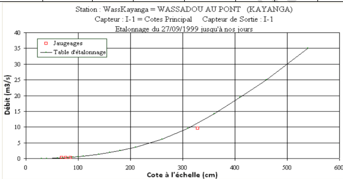
Figure 6: Calibration curve of the Kayanga at the Wassadoubridge
