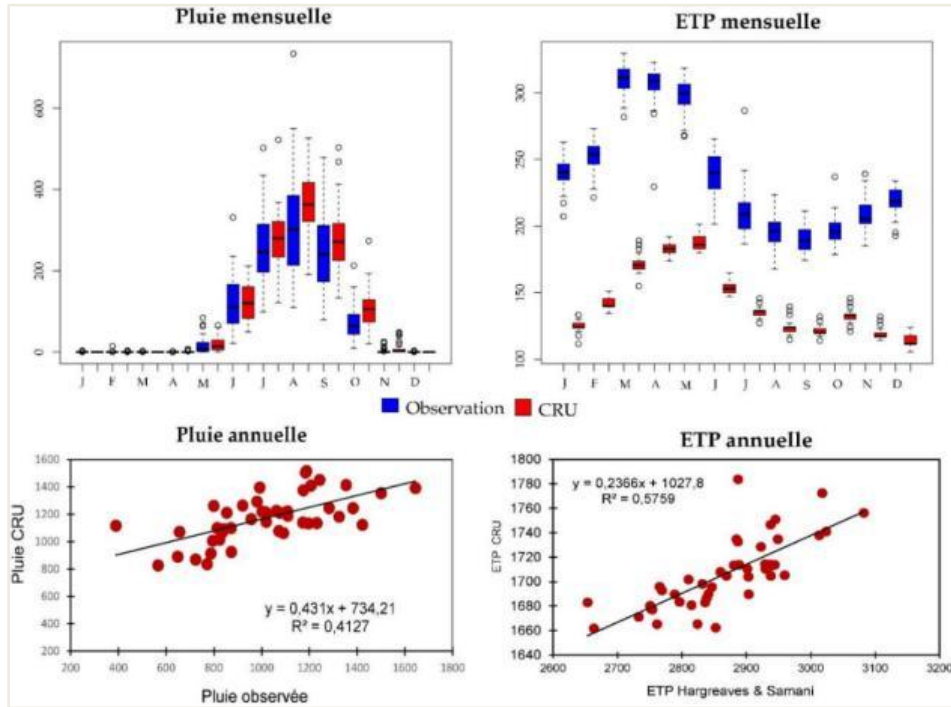
Figure 8. Validation of CRU rainfall and ETP data with station data Kolda reference
