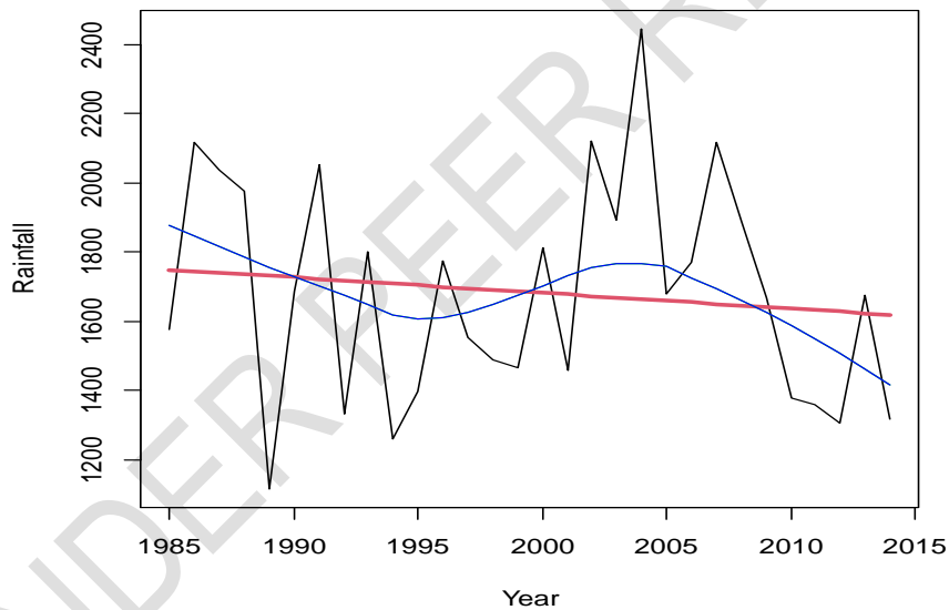
Fig. 1. Lowess curve for Rainfall
