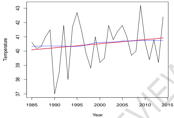
Fig. 2. Lowess curve for annual maximum Temperature
