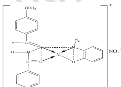
Figure 3: The proposed geometry of mixed ligand complexes for L1 and L2 where, M=Cu(II), and Ni(II)
