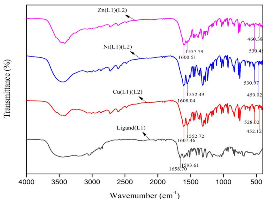
Figure 1: IR Spectra of the ligand L1, and its Mixed Ligand Complexes with L2.
