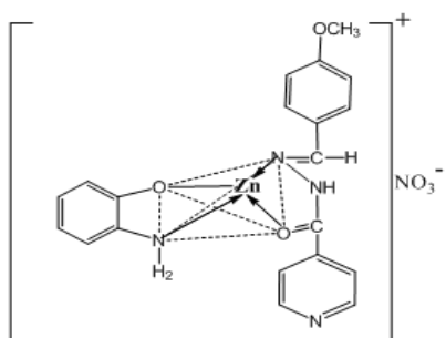
Figure 4: The proposed geometry of mixed ligand complexes for L1 and L2
