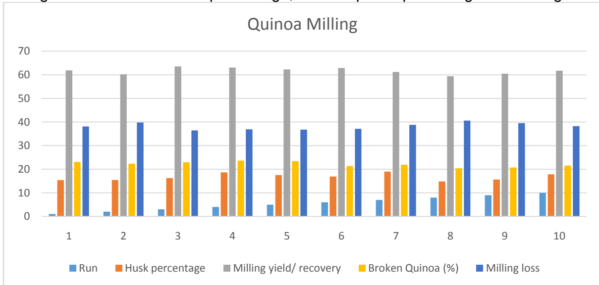
Graph 1: Effect of milling on its fractions under different runs of pearling
