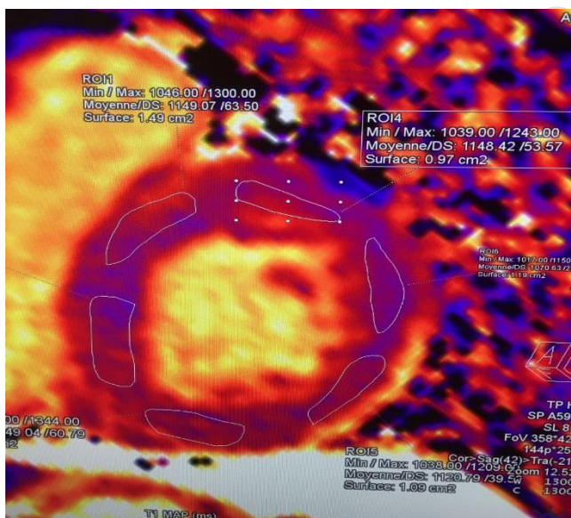
Figure 6. T1 mapping cartography > 1100 ms diffusion: myocardial infiltration.
