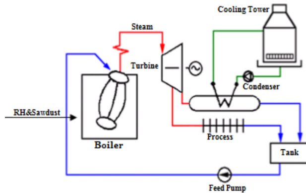
Fig. 2. Schematic diagram of electrical energy generation
