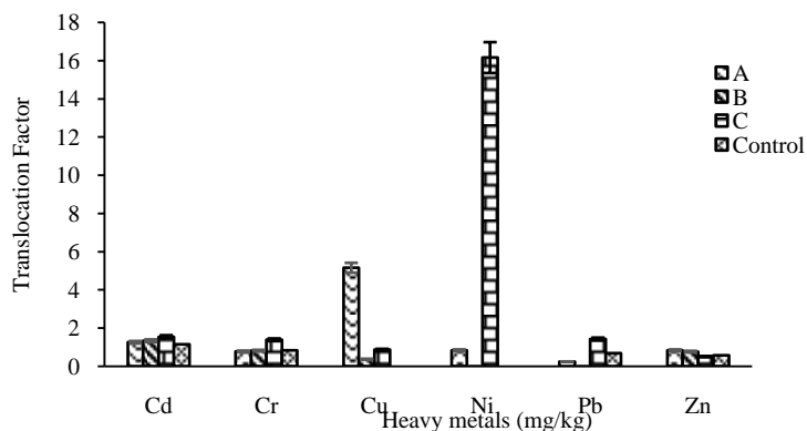
Fig. 5. Mean Translocation Factor of Heavy metals in E. crassipes . The descending order of Translocation factor ranged from the maximum to the minimum at the sampling points is as follows; Ni>Cu>Cd>Pb>Cr>Zn.
