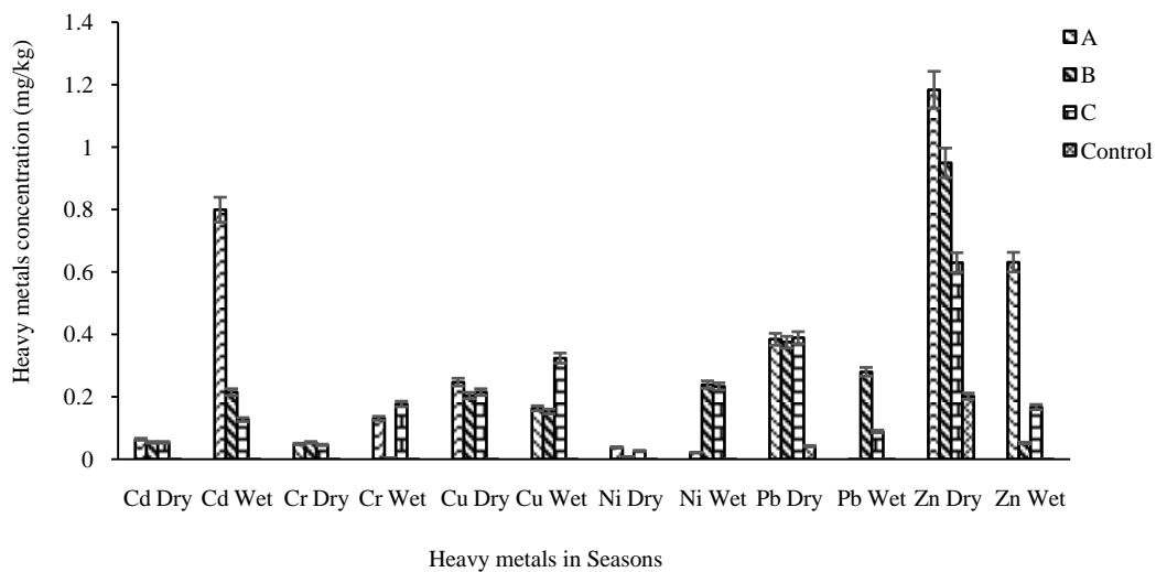
Fig. 2. Mean Concentration of heavy metals at the sampling points during dry and wet seasons.
