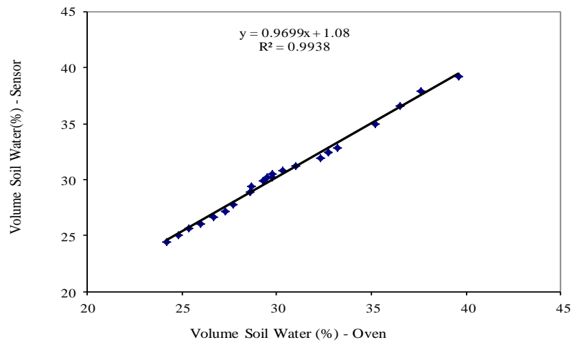
Fig. 5. Soil moisture sensor calibration curve
