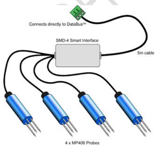
Fig. 2 (a). 4 x MP406 Probes with Smart Interface
