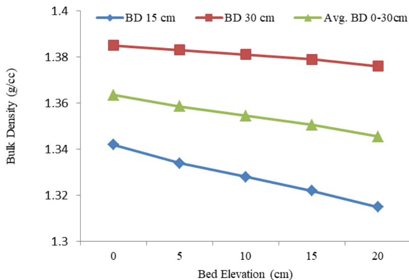
Fig. 3. Variation of bulk density at 24.85% moisture content in rabi 2018-19
