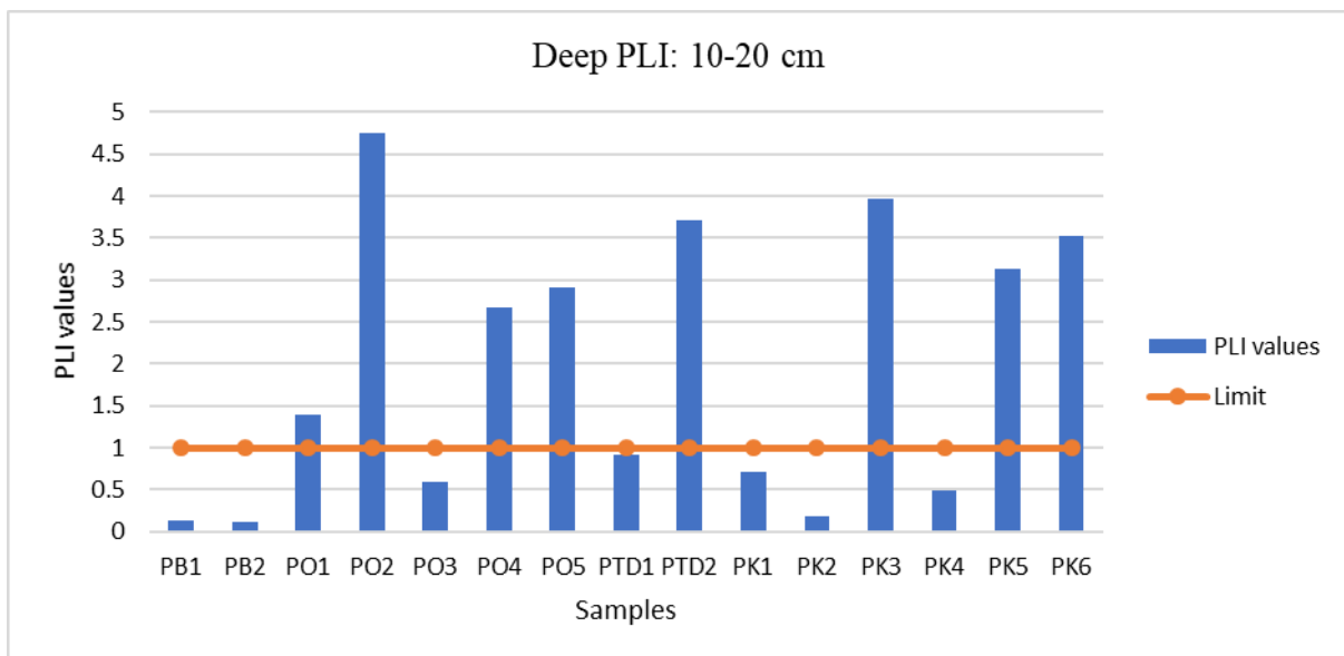
Figure 9: Pollution index at depth (10-20 cm)
