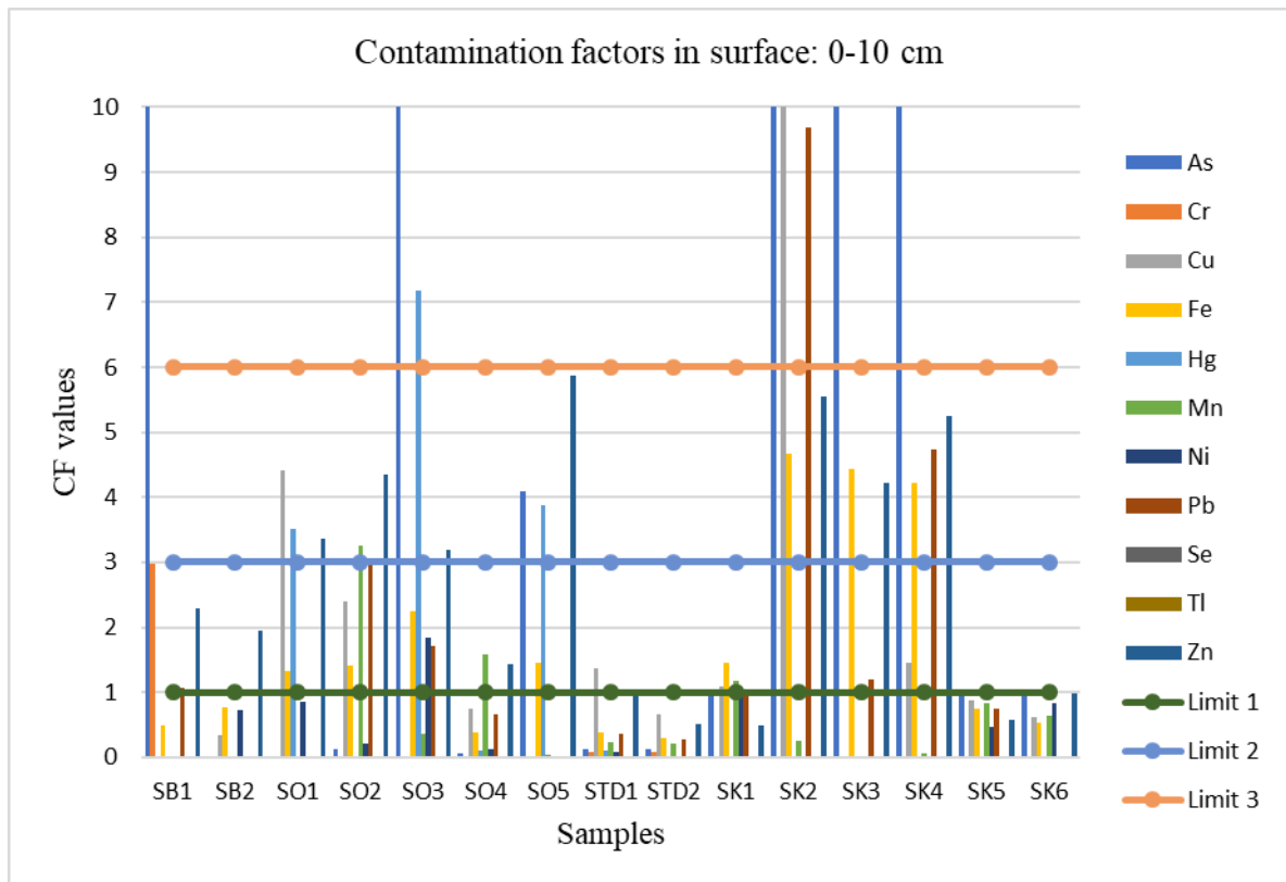
Figure 4: Variations in contamination factors in the 0-10 cm soil profile
