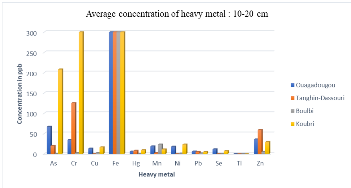
Figure 3: Average concentrations of heavy metals in the 10-20 cm profile
