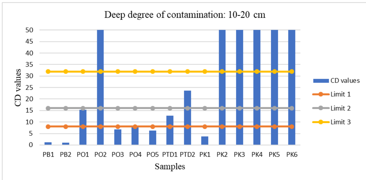
Figure 7: Variations in degrees of contamination in the 10-20 cm profile of
