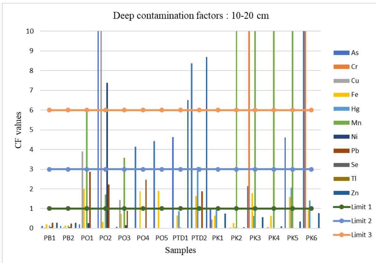
Figure 5: Variations in contamination factors in the 10-20 cm soil profile
