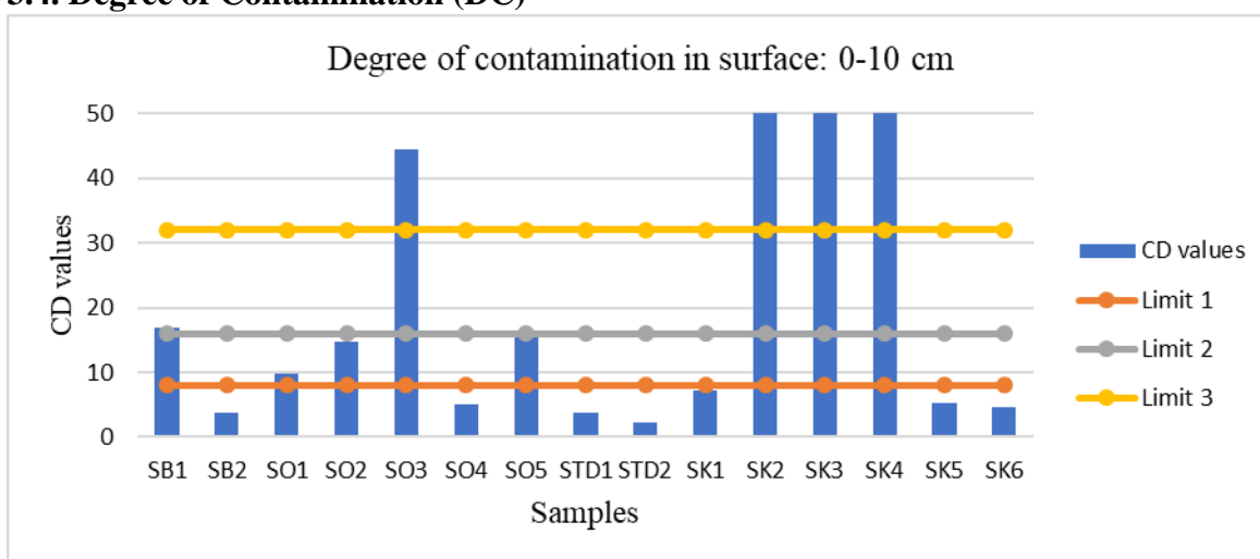
Figure 6: Variations in contamination degrees in the 0-10 cm soil profile
