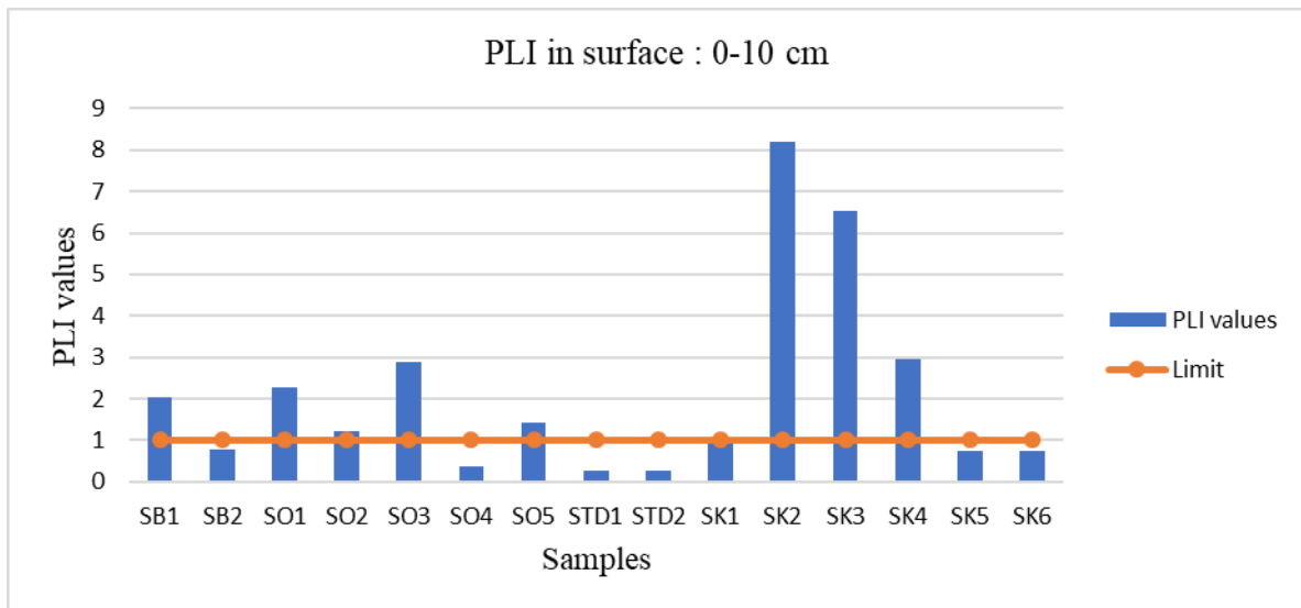
Figure 8: Surface pollution index (0-10 cm)
