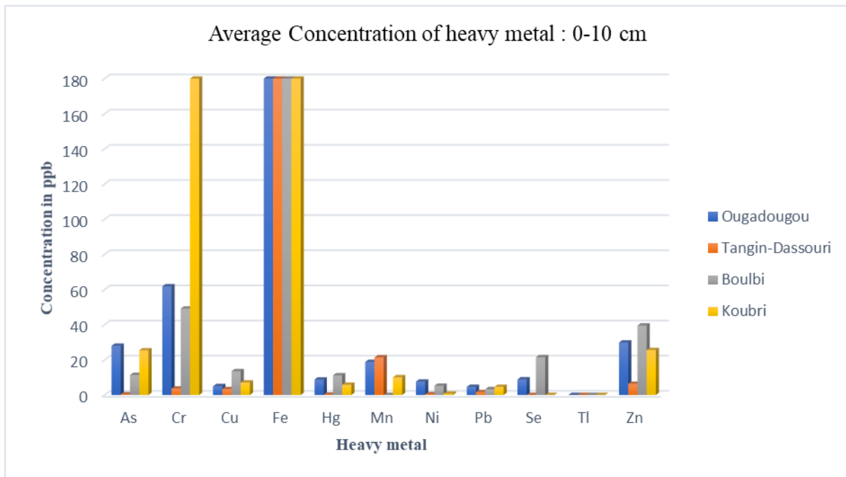
Figure 2: Average concentrations of heavy metals in the 0-10 cm profile
