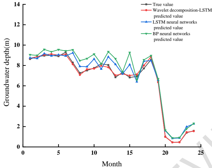
Fig.9 Comparison of the prediction results of the LuWangfen Town wavelet decomposition-LSTM model with other models
