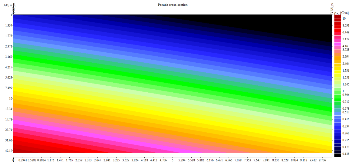
Fig 11. Pseudo cross section VES 3
