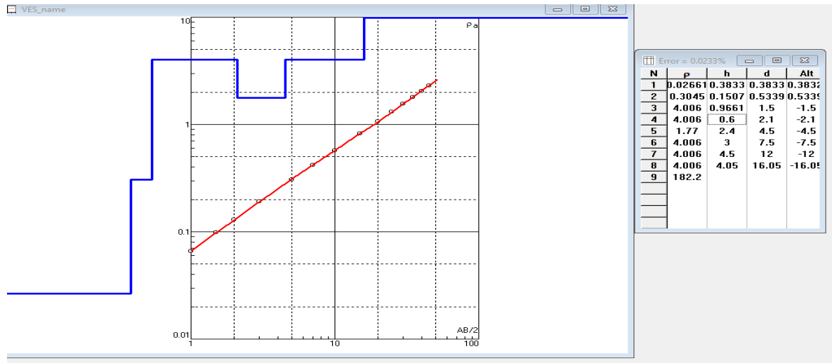
Fig 6 Inverted Model Layer for VES 1: Ikarama Oil Spill Site
