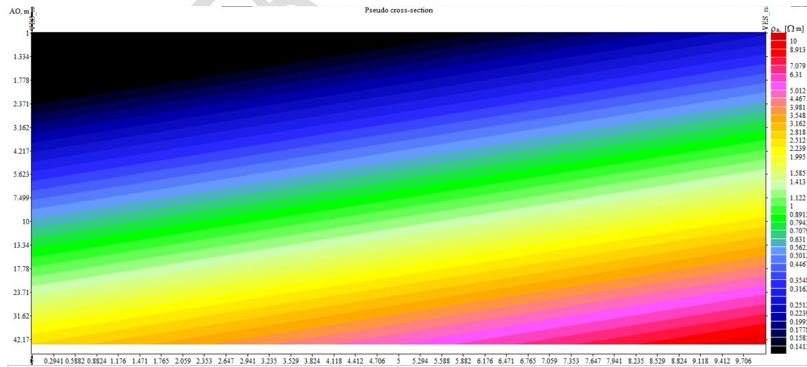
Fig 10. Pseudo cross section VES 2
