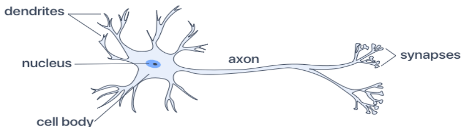
Figure 1 Biological Neuron
