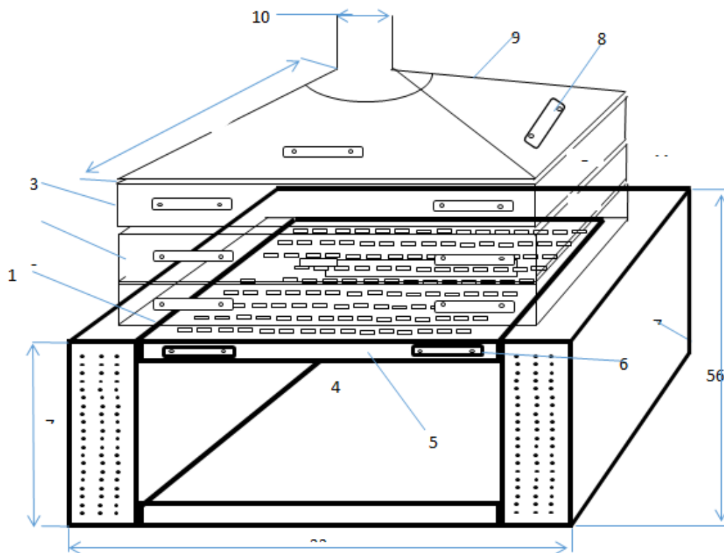
Fig. 1. Schematic diagram of a modified smoking kiln showing the front view (all dimensions are in
