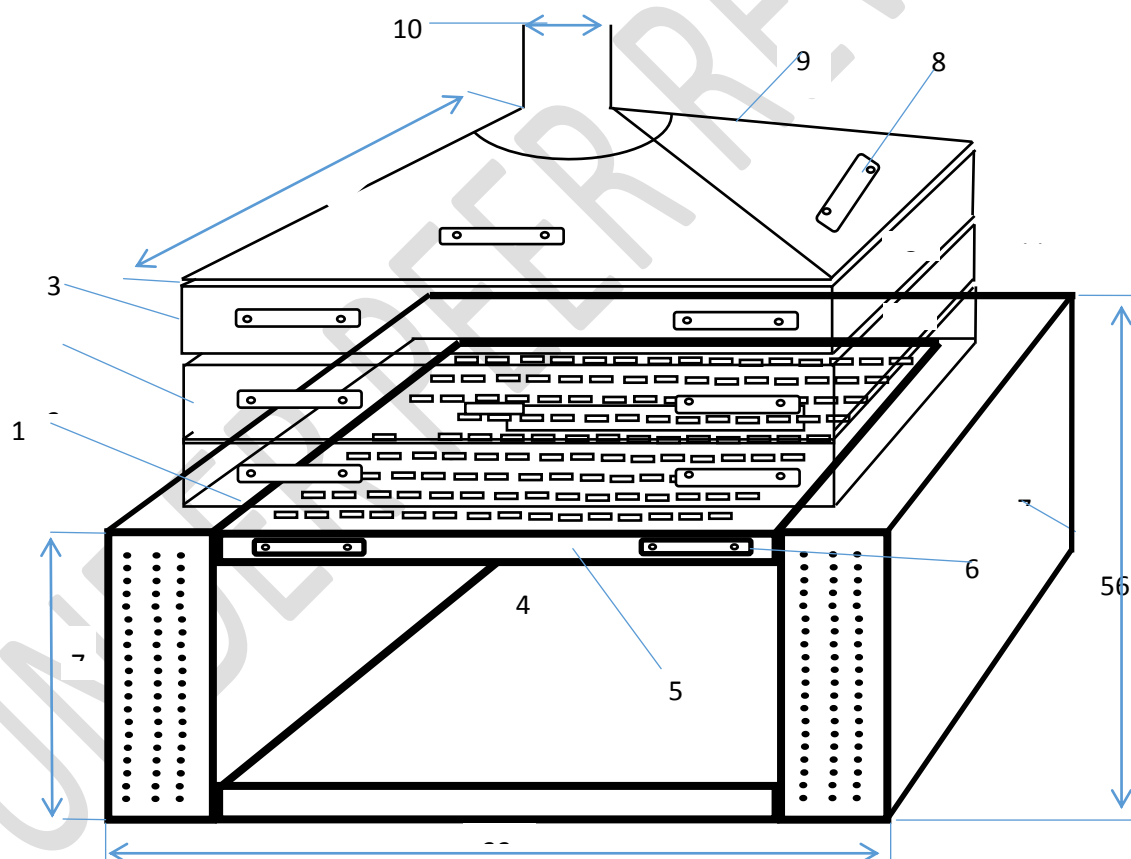
Fig. 1A. Schematic diagram of a modified smoking kiln showing the front view (all dimensions are in
