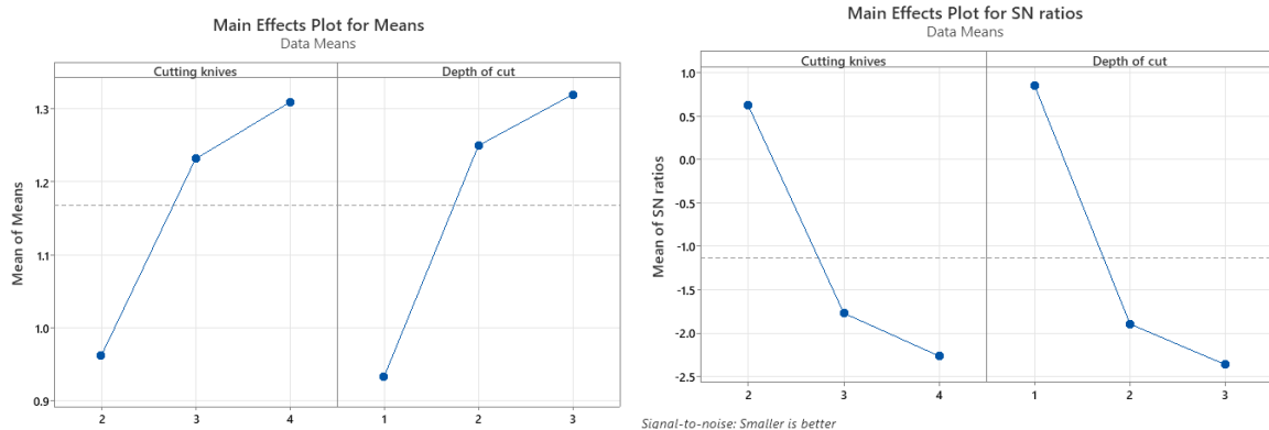
Fig. 4. Main Effects Plot for S/N Ratios on Data Means: Pine Total Cutting energy (TCE)
