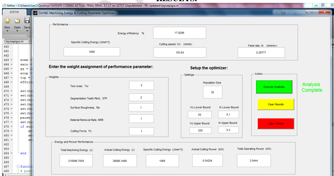
FIGURE. 9 SIMULATION RUN, COMPLETE, IMAGE OF THE IEUCPPTM DISPLAYING RESULTS.
