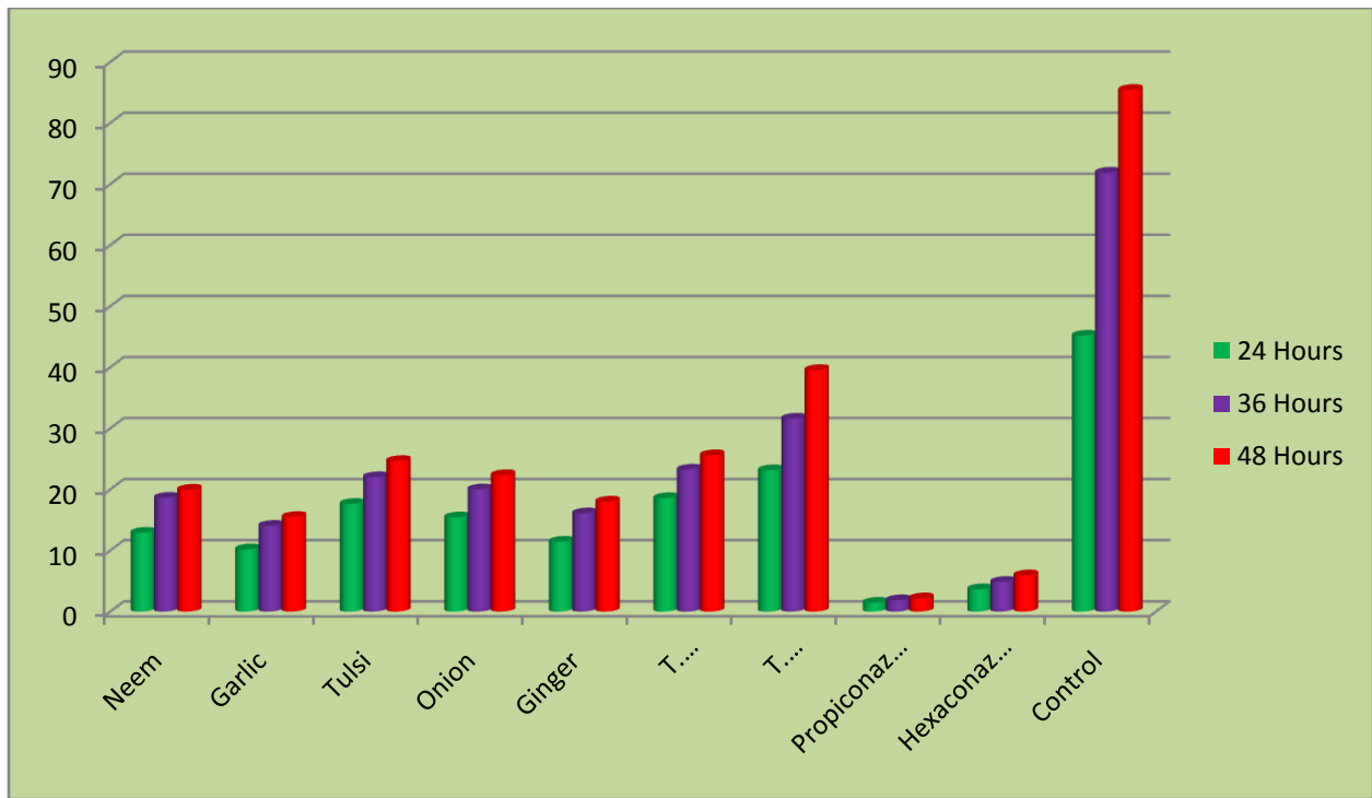
Fig.1: Effect of botanicals, bio-agents and fungicides against R. solani on mycelial growth at 24, 36 and 48 hours.
