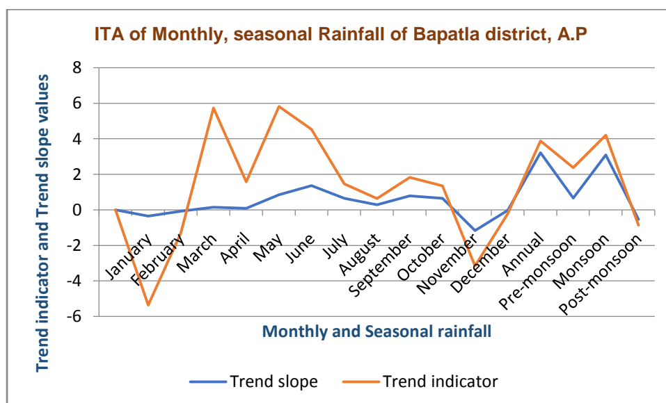
Fig 3. Trend indicator and Trend slope of Innovative trend Analysis
