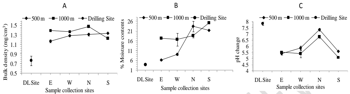
Figure 1: Effect of crude oil contamination on (A) bulk density ( \text{mg}\cdot\text{cm}^{-3} ), (B) % moisture content and (C) soil pH in the samples collected from different sites. The vertical bars represent the mean standard error. The \pm SEM values in the error bars for (A) and (B) are shown as a multiple of 10. *** represent the significance at 0.1% level of probability.
