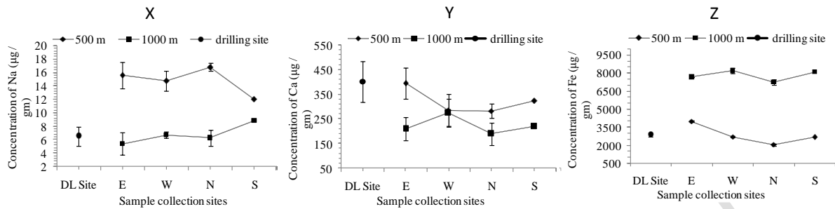
Figure 4: Effect of crude oil contamination on (X) sodium concentration ( \mu\text{g/g} ), (Y) soil Ca concentration ( \mu\text{g/g} ) and (Z) total iron ( \mu\text{g/g} ) in the samples collected from different sites. The vertical bars represent the mean standard errors. The \pm\text{SEM} values in the error bars are shown as a multiple of 10. *** Significant at 0.1% level of probability.
