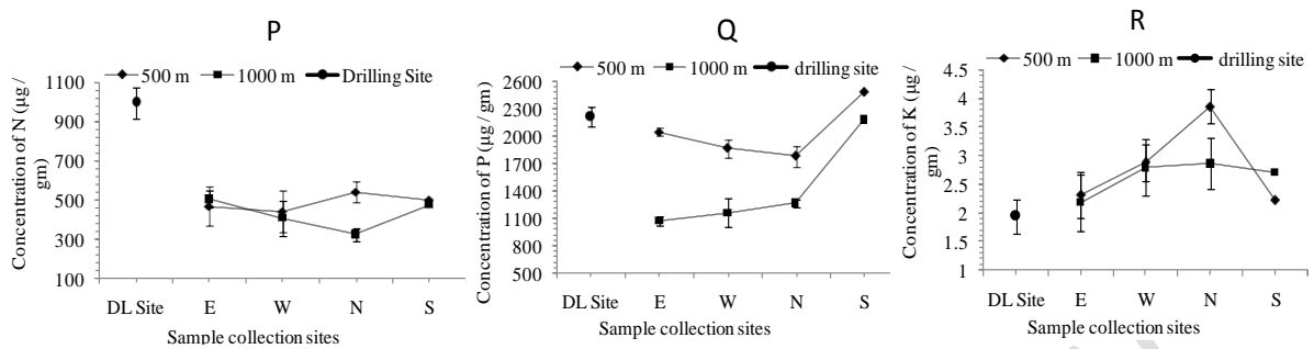
Figure 3: Effect of crude oil contamination on (P) soil nitrogen ( \mu\text{g/g} ), (Q) available phosphorous ( \mu\text{g/g} ) and (R) potassium concentration ( \mu\text{g/g} ) in the samples collected from different sites. The vertical bars represent the mean standard errors. The \pm\text{SEM} values in the error bars are shown as a multiple of 10. *** Significant at 0.1% level of probability.
