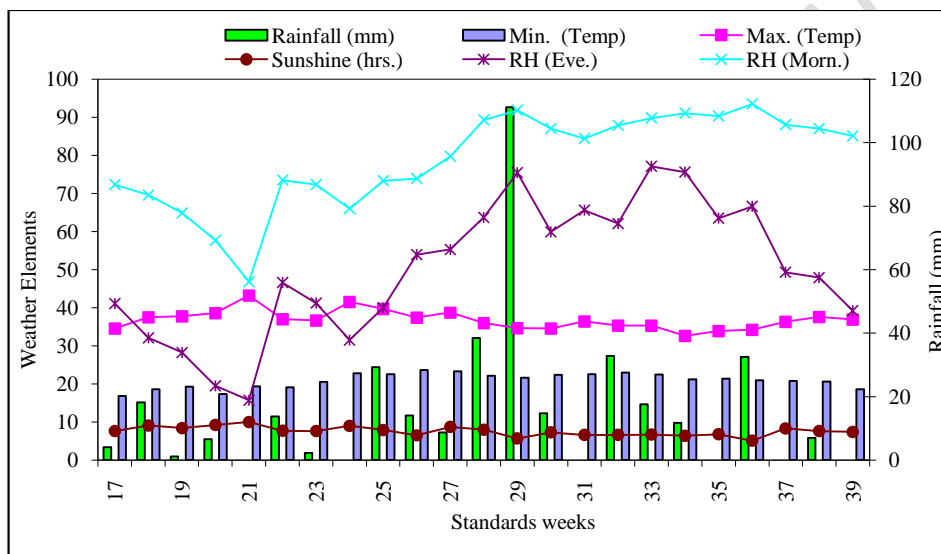
Fig. 1: Mean weekly meteorological data during crop season (2020)
