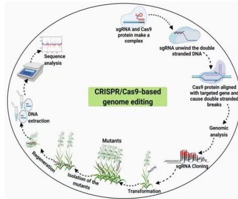
Figure 2. Cas9-based genome editing mechanism. The Cas9 gene-editing system includes the sgRNA and Cas9 protein complex, sgRNA-induced DNA unwinding, Cas9-induced gene cutting, analytic tools, cloning, transformation, and more. This editing technique does not need any external elements.
