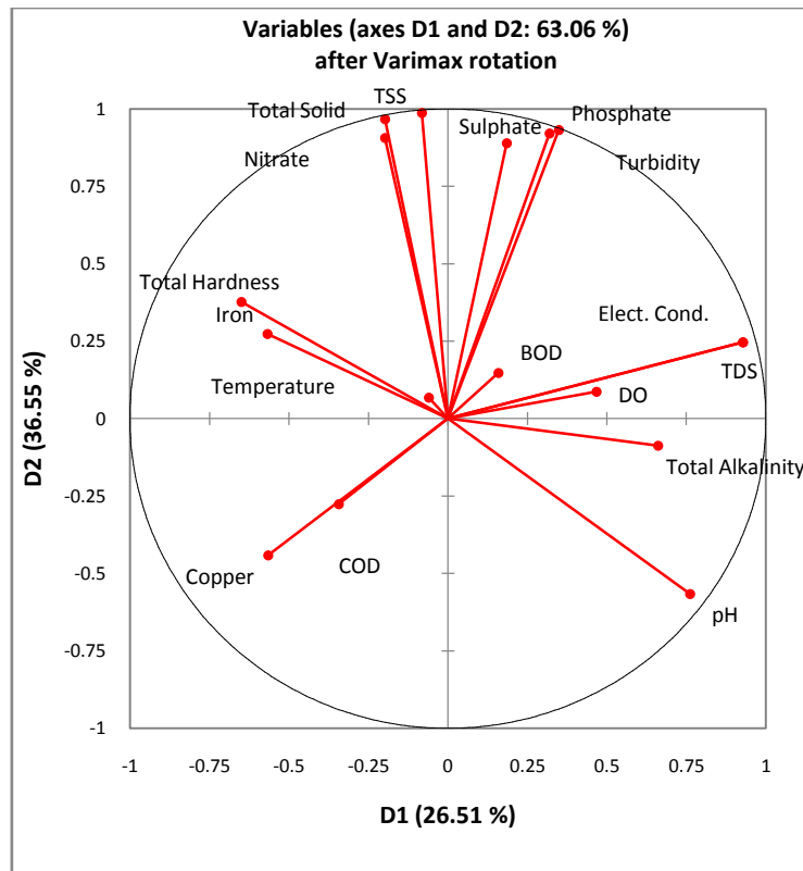
Figure 2: Biplot showing the physicochemical parameters on principal component 1 and 2
