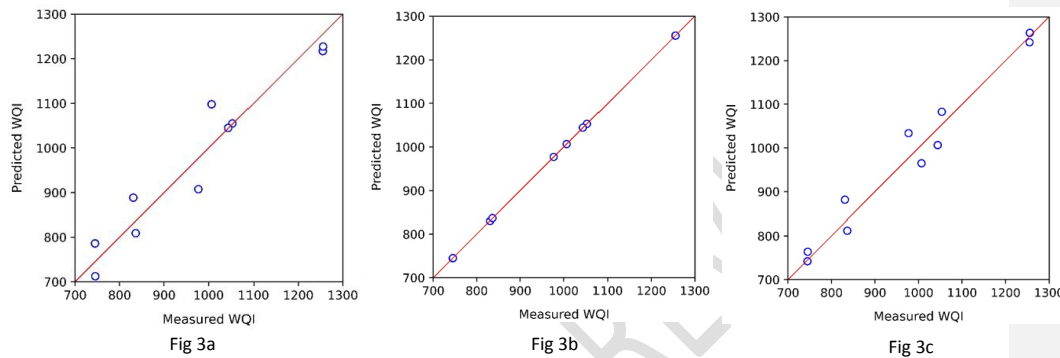
Fig 3: Model Prediction Comparison
