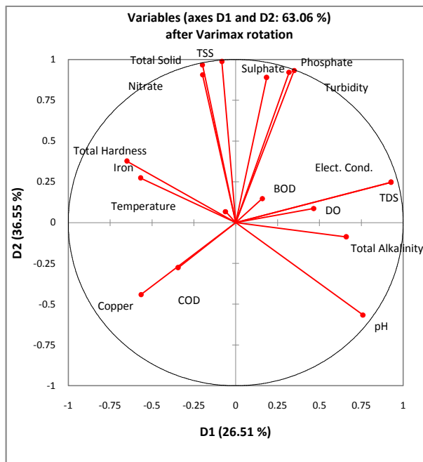
Figure 2: Biplot showing the physiochemical parameters on principal component 1 and 2
