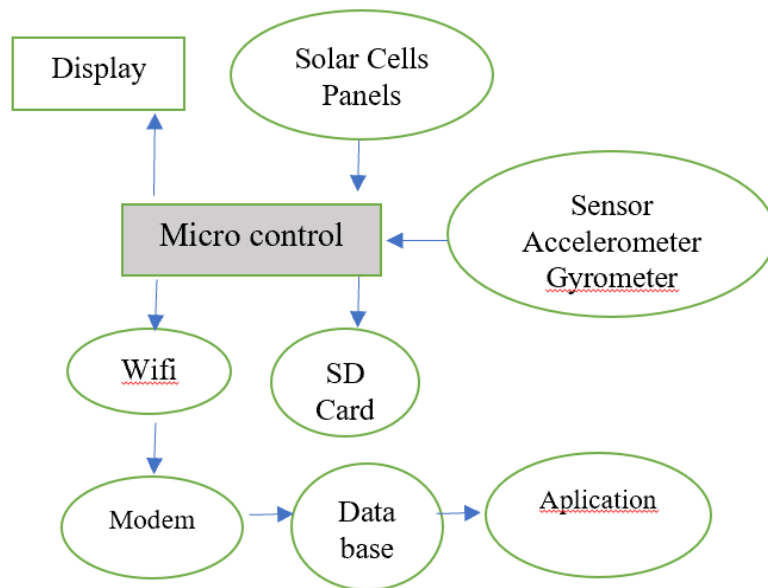
Fig. 3. Landslide Early Warning System Diagram
