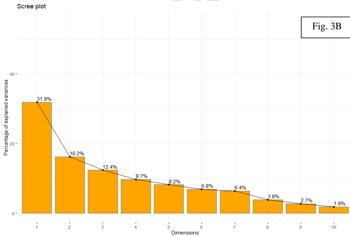
Fig. 3 (A&B): Scree plot showing percentage of explained variance for root architectural traits of introgression lines under two soil P gradient conditions during Kharif-2020; Fig.3A: percentage of explained variance under low soil P; Fig.3B: percentage of explained variance under normal soil P; Note: 1 to 10 number = component numbers
