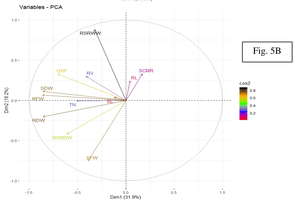
Figure 5: A and B showing the PCA Biplot for genotype clustering and PCA variable showing the contribution of the root traits in PC1 and PC2 on the axes under normal soil P during Kharif-2020
