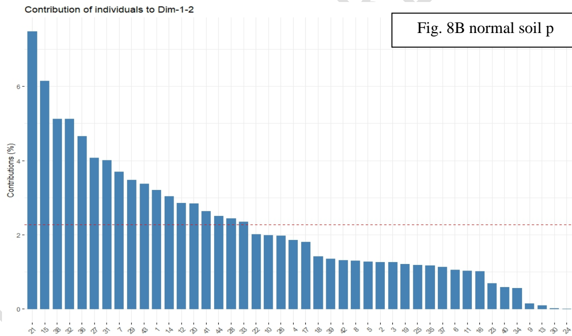
Figure 8: A and B showing the PCA graphs for individual genotype contributing to the variability through first two PCs for root architectural traits of introgression lines under two soil P gradient conditions during Kharif-2020
