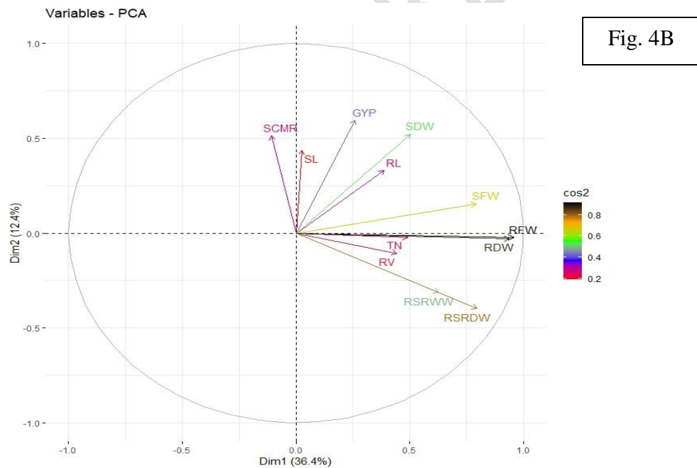
Figure 4: A and B showing the PCA Biplot for genotype clustering and PCA variable showing the contribution of the root traits in PC1 and PC2 on the axes for introgression lines under low soil P gradient conditions during Kharif -2020
