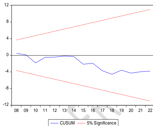
Figure 1: Cumulative Sum Test
