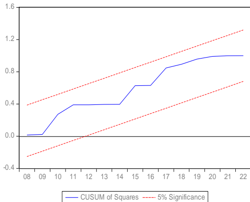
Figure 2. Cumulative Sum of Squares Test
