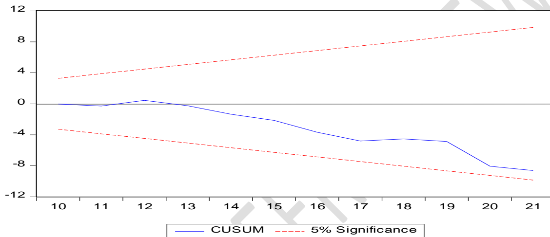
Figure 4: Cumulative Sum Test for Stability
