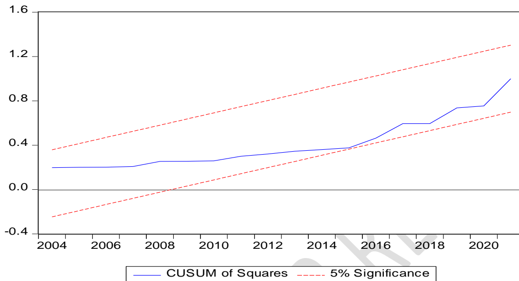
Figure 5: Cumulative Sum (CUSUM) of squares test for stability
