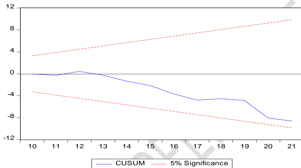
Figure 4: Cumulative Sum Test for Stability
