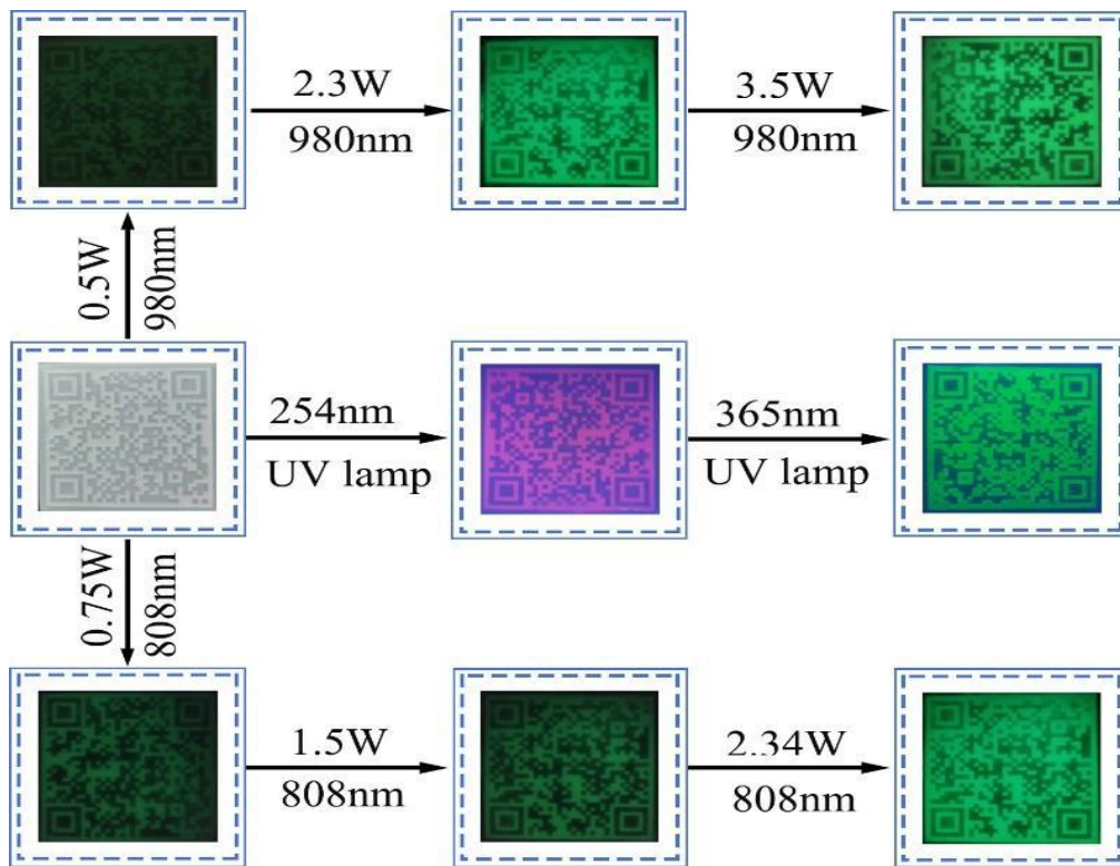
Figure 10: Design of \text{La}_4\text{GeO}_8\text{Eu}^{2+/3+}, \text{Er}^{3+} multi-modal anti-counterfeiting QR code.
