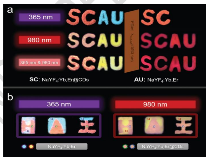
Figure 8(a,b) shows the luminescent anti-counterfeiting application patterns of \text{NaYF}_4:\text{Yb,Er@CDs} nanocomposite material and \text{NaYF}_4:\text{Yb,Er} phosphor.
