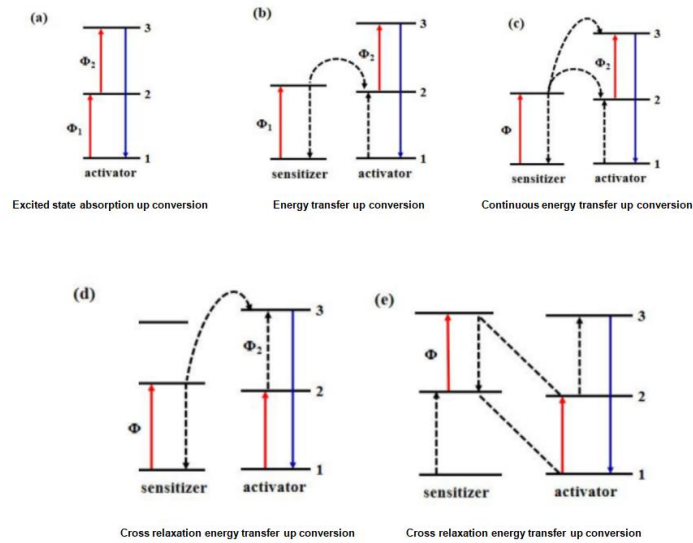
Figure 1 Upconversion Luminescence Processes (a-e)[4]
