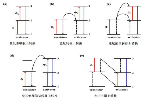
Figure 1 Upconversion Luminescence Processes (a-e)[4]
