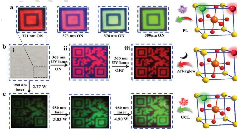
Figure 9(a,b,c): shows the multi-modal luminescent anti-counterfeiting pattern of CaTiO 3 :Pr 3+ ,Er 3+ .
