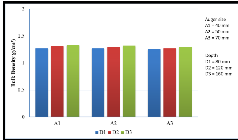
Fig. 6 Effect of auger size and depth on bulk density
