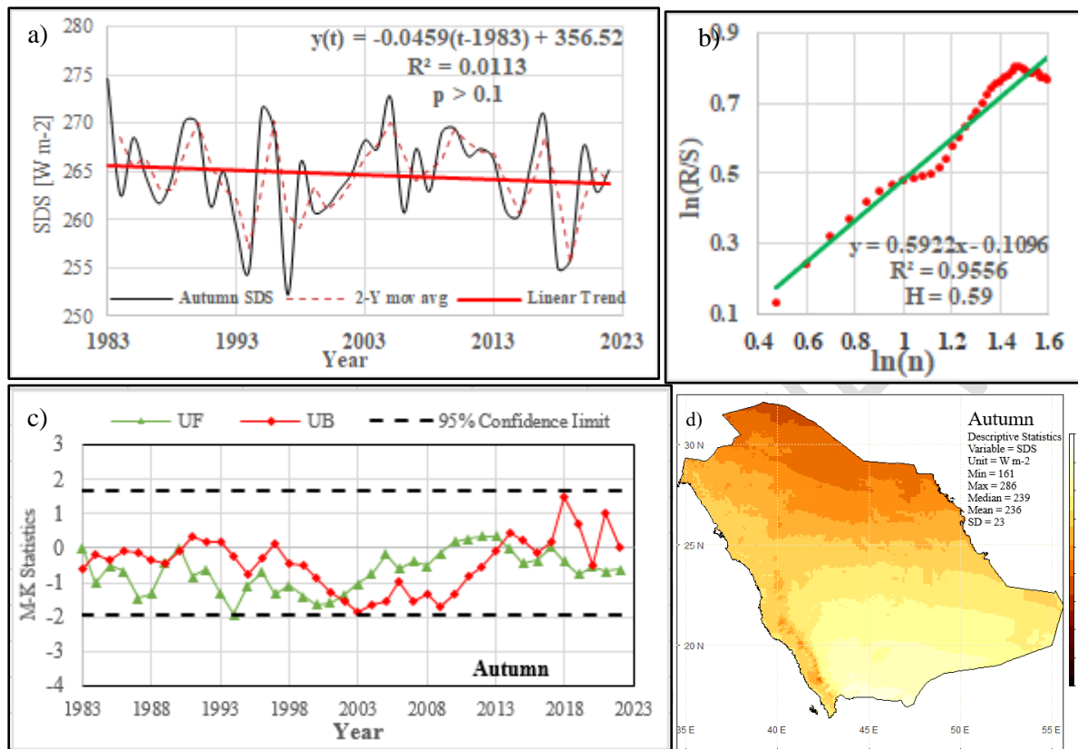
Figure 5: Variation of SDS Radiation in Saudi Arabia during Autumn Season
