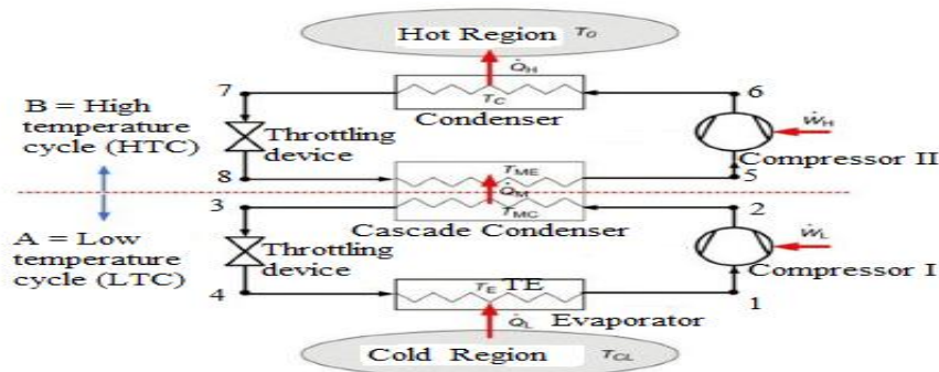
Figure 1 Schematic diagram cascade refrigeration system
