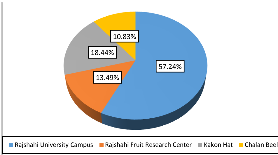
Fig. 1. Site-wise abundance of leaf litter and subsoil arthropods
