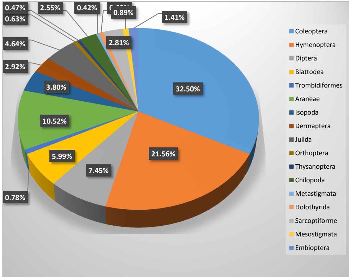
Fig. 3. Order-wise abundance of leaf litter and subsoil arthropods.
