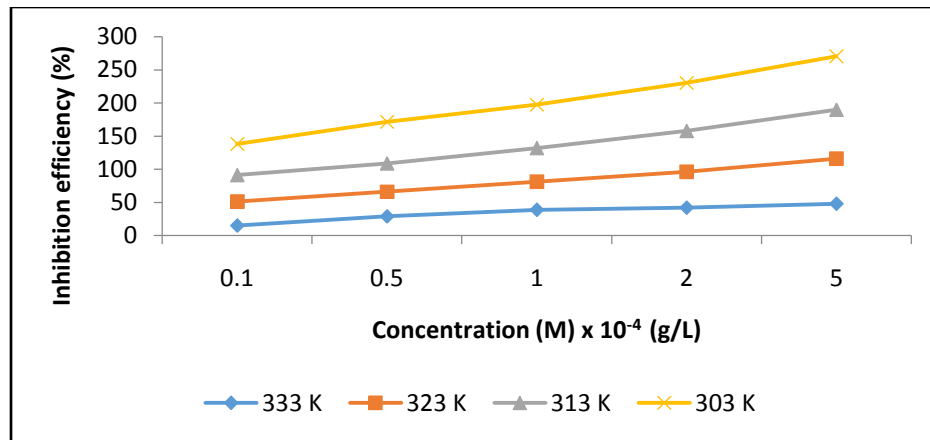
Figure 1: Effect of semi-pure extract of C. nitida (Mb4) on the corrosion inhibition efficiency of mild steel at different temperatures.
