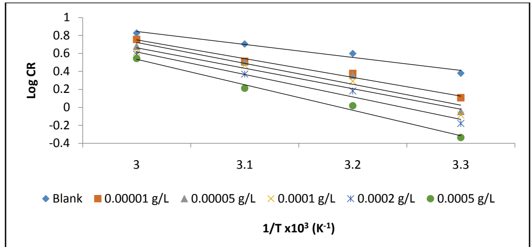
Figure 5: Arrhenius plot for mild steel coupons in 1 M HCl in the absence and presence of different concentrations of Mb4.
