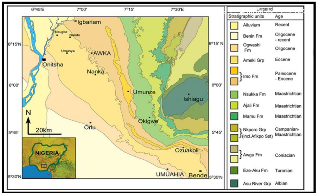
Fig. 2: Geologic map of southeastern Nigeria (Short and Stauble, 1967)
