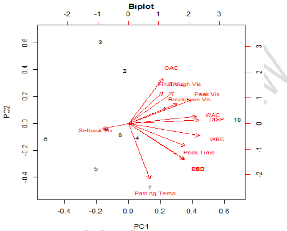
Fig 1. Loading plot with first and second components of the principal component analysis of the variables of the functional and pasting attributes of the flour samples
