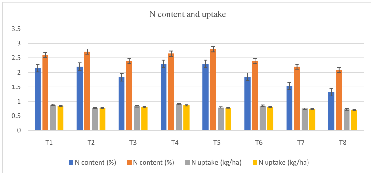
Figure 1- Effect of organic manures and natural farming on N content and uptake by carrot roots and leaves
