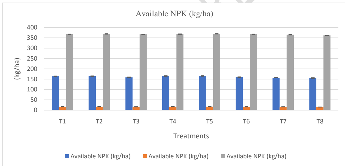
Figure 2- Effect of organic manures and natural farming on NPK in soil after harvest.
