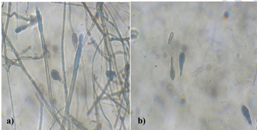
Figure 2. Microphotographs of conidia of Alternariasolani at 100X
