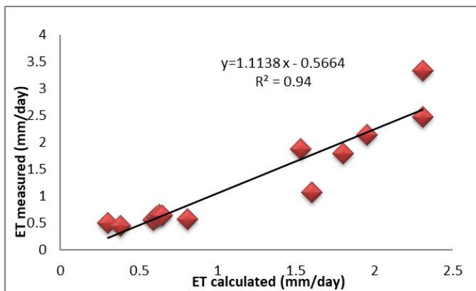
Fig.2. ET_c Lysimeter versus ET_c by Penman-Monteith method
