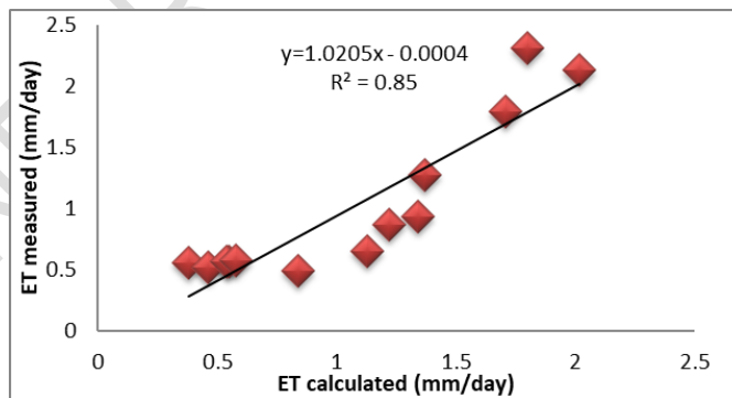
Fig. 4. ET_c lysimeter versus ET_c by Blaney-criddle method
