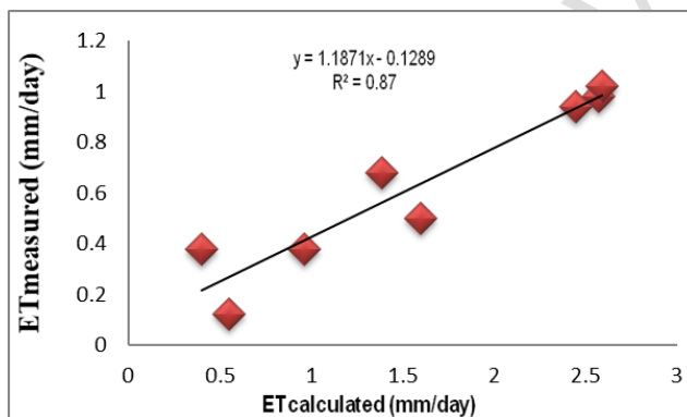
Fig 3. ET_c Lysimeter versus ET_c by Hargreaves method
