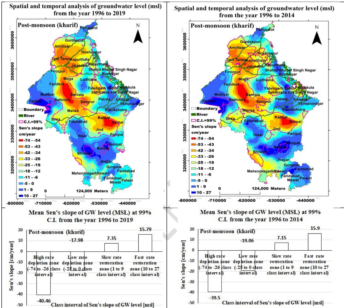
Figure 5(d). Spatial and temporal analysis of groundwater level (MSL) and Sen's slope for post-monsoon (kharif) season from the years 1996 to 2019 and 1996 to 2014.
