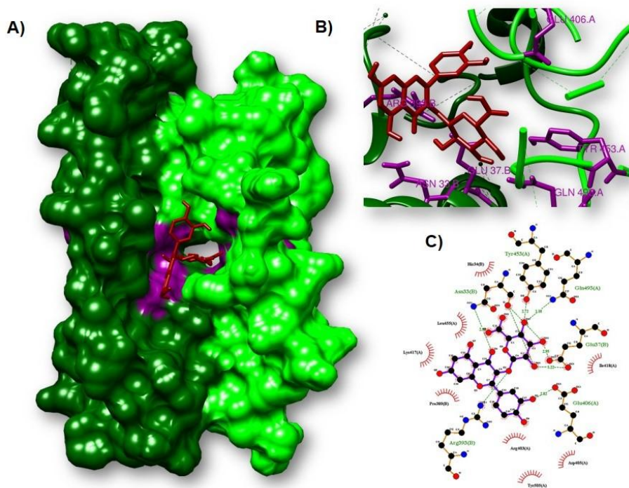
Figure 7: Molecular coupling of the Myquelianine ligand (red) with the Spike/ ACE2 complex obtaining binding free energy of -8.5 kcal.mol -1 . A) Site of interaction of the protein-ligand complex. B) 3D conformation of the active site of the binding of the myquelianine compound with the Spike/ACE2 complex. C) 2D scheme showing hydrogen bonds and hydrophobic interactions.
